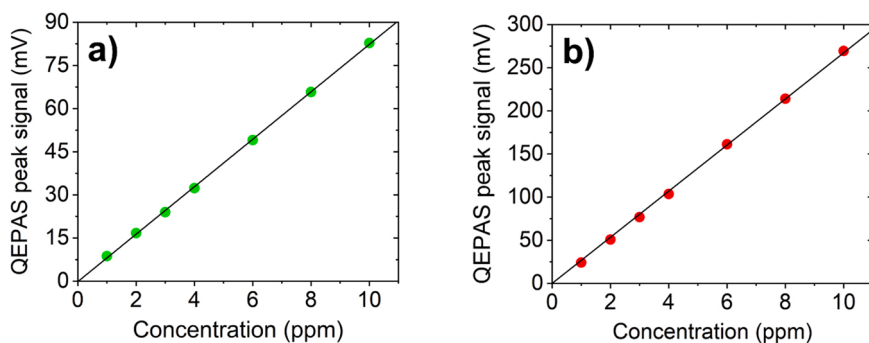
Fig. 4. (a) Peak values measured for each methane concentration (green dots). The black solid line is the best linear fit of the experimental data. (b) QEPAS peak signal as a function of N 2 O concentration (red dots) with the corresponding best linear fit (black line).
