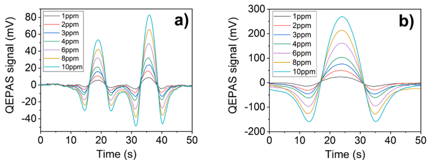
Fig. 3. a) QEPAS spectral scans measured for different CH 4 in standard air concentrations. b) N 2 O QEPAS scans measured for 7 different N 2 O concentrations in standard air.
