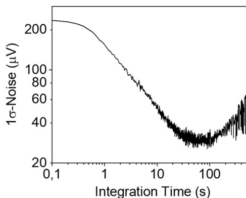
Fig. 5. Allan-Werle deviation plot of the QEPAS signal as a function of the integration time. For a 10 s integration time, the 1 \sigma -noise level can be lowered to ~ 50 \mu V.
