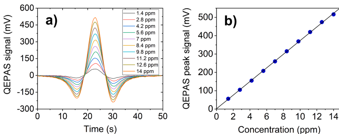
Fig. 7. (a) 2f -QEPAS spectra collected by varying the \text{NH}_3 concentration within the gas cell. (b) QEPAS peak signals extracted from spectral scans reported as function of \text{NH}_3 concentration (blue dots). The performed best linear fit is superimposed to the collected data (black line).
